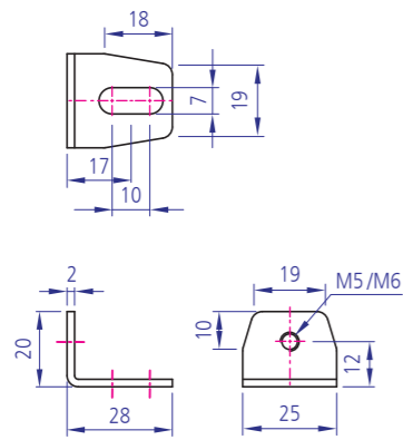
YKBK-S T28*25(M5,M6) Code : YKBK-ST2825
