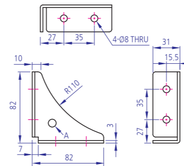
YKBK-S G40*80(HOLE) Code : YKBK-SGT4080H
