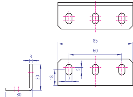
YKBK-S G30*85 Code : YKBK-SG3085
