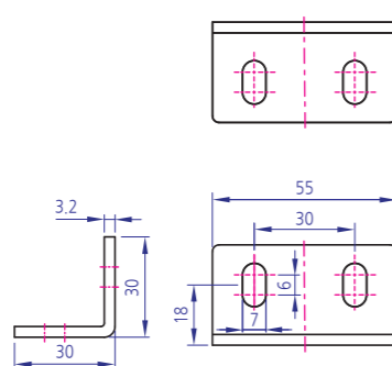
YKBK-S G30*55 Code : YKBK-SG3055
