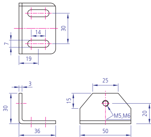
YKBK-S T30*50(M5,M6) Code : YKBK-ST3050
