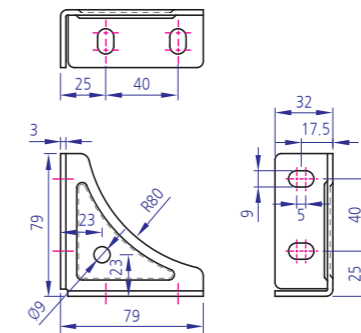
YKBK-S G40*80(장공) Code : YKBK-SGT4080L
