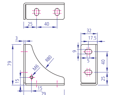
YKBK-S G40*80(장공) T40*80(P15*15) Code : YKBK-SGT4080A
