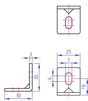
YKBK-S G30*25 Code : YKBK-SG3025
